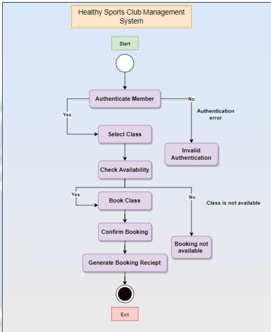
Figure 2: Activity Diagram
