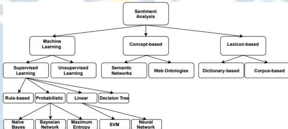
Figure 8: Sentiment classification techniques
