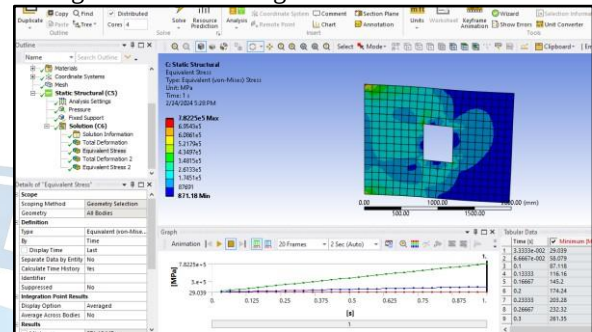
Fig 19. Equivalent stress The equivalent stress of a square cut plate shows the maximum stress value as 7.8225e5 MPa and the minimum stress value as 871.18 MPa.
