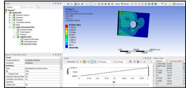
Fig 6. Equivalent stress
