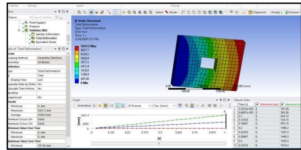
Fig 12. Total displacement
