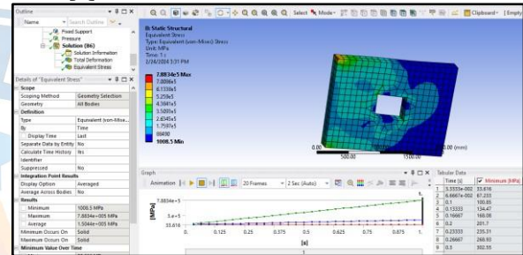
Fig 13. Equivalent stress
