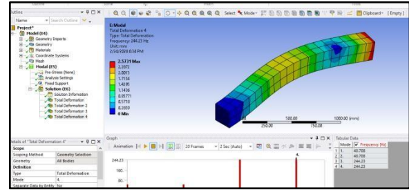
Fig 31. Second frequency
